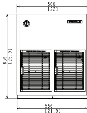
WATER-COOLED
