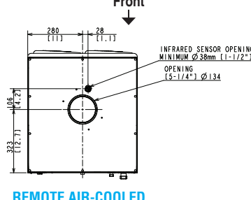
REMOTE AIR-COOLED
